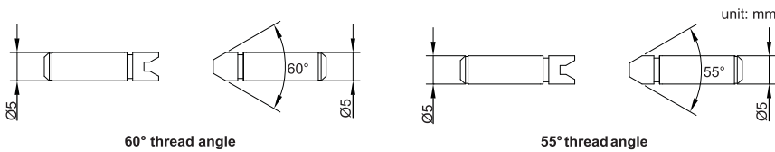
60° thread angle
