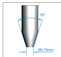
HSM1A indenter
