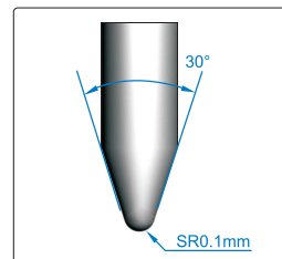
HSM5D indenter
