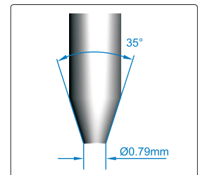
HS1A indenter
